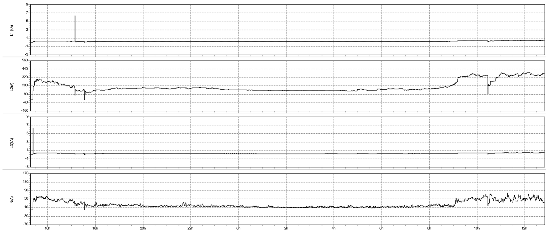
Fig.3 Shows the current on three phases for 22 hours from 15/03/2023 15:17 pm to 16/03/2023 12:50 pm
