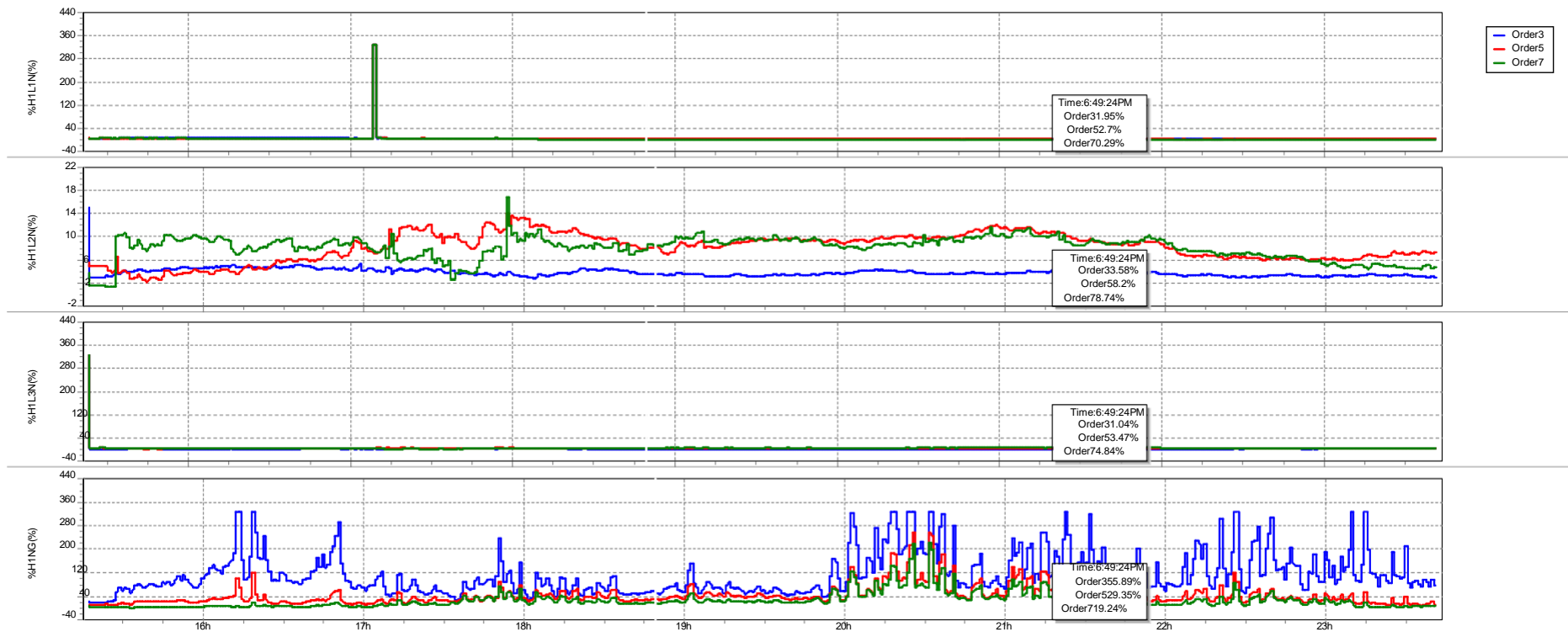
Fig.15 Shows the THD (Current Harmonics) for 3 rd , 5 th and 7 th order for 22 hours from 15/03/2023 15:17 pm to 16/03/2023 12:50 Inference:
